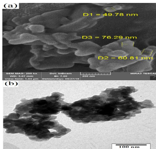
Fig 3. a) SEM and b) TEM of \text{SrCO}_3 Nanostructures in Sample Three
