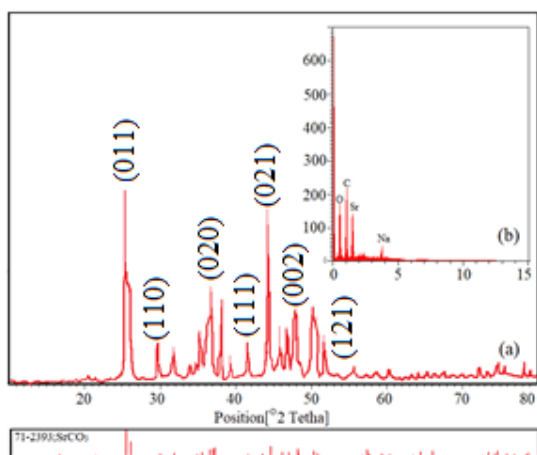
Fig 2. XRD Patterns of \text{SrCO}_3 Nanostructures for Sample Three after Calcination at Temperature of 150 °C
