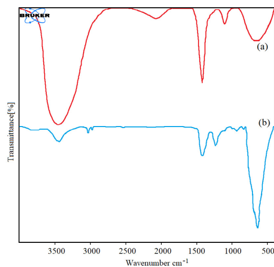
Fig 1. FT-IR Spectra of \text{SrCO}_3 Nanostructures; a) Room Temperature, b) after Calcination at Temperature of 150\text{ }^{\circ}\text{C}
