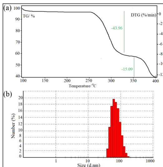
Fig 4. a) TGA Analysis and b) DLS Analysis of \text{SrCO}_3 Nanostructures in Sample Four
