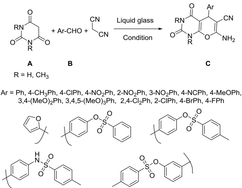
Scheme 1. Preparation of pyrano[2,3-d]pyrimidine derivatives.
