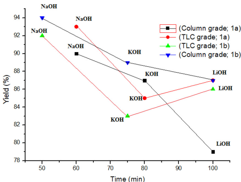
Figure 1. Preparation of 7-Amino-2,4-dioxo-5-phenyl-1,3,4,5-tetrahydro-2H-pyrano[2,3-d]pyrimidine-6-carbonitrile: Effect of liquid glass composition (37% solution in water, MOH bases; silica (TLC and column grade)). 1a: Si/M ratio: 1.5; 1b: Si/M ratio: 1.
