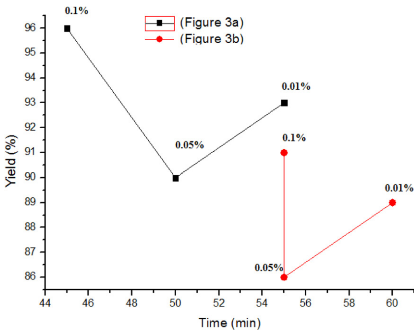
Figure 3. Effect of MgO (3a) ZnO (3b) and impurity on the liquid glasses (NaOH; silica TLC grade; 37% solution in water, Si/Na ratio: 1.5) catalyzed preparation of 7-amino-2,4-dioxo-5-phenyl-1,3,4,5-tetrahydro-2H-pyrano[2,3-d]pyrimidine-6-carbonitrile.
