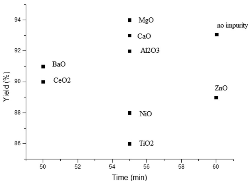
Figure 2. Effect of different metal oxide impurities on the liquid glasses (NaOH; silica TLC grade; 37% solution in water, Si/Na ratio: 1.5) catalyzed preparation of 7-amino-2,4-dioxo-5-phenyl-1,3,4,5-tetrahydro-2H-pyrano[2,3-d]pyrimidine-6-carbonitrile.
