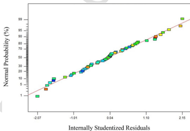
Fig. 3. The normal probability vs. residuals plot by final fitted model.
