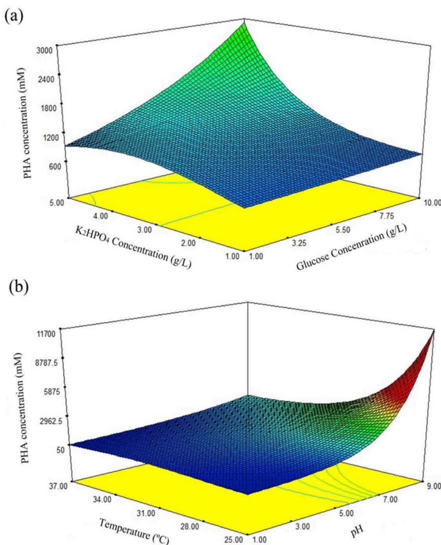
Fig. 4. Response surface of PHA concentration. (a) constant level of \text{NH}_4\text{Cl} (1 g/L), pH (9), and temperature (30 °C) and (b) constant level of glucose (10 g/L), \text{K}_2\text{HPO}_4 (5 g/L), and \text{NH}_4\text{Cl} (1 g/L).
