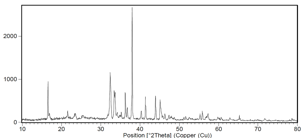
Fig. 2. XRD pattern of zirconium metal-organic framework nanostructures
